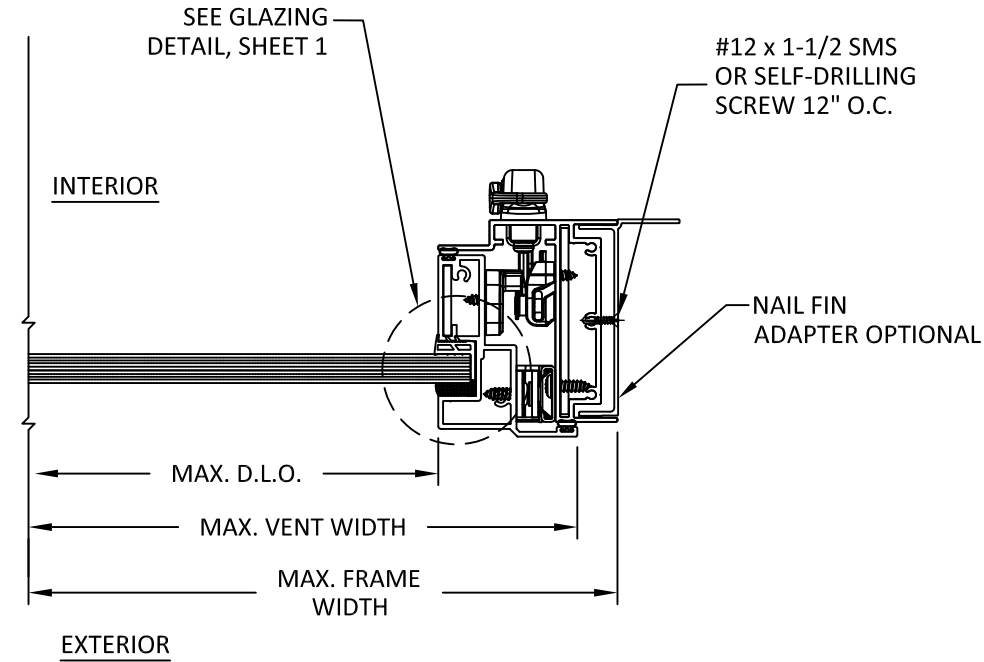
B 4 HORIZONTAL SECTION RIGHT JAMB DETAIL NAIL FIN ADAPTER SHOWN
