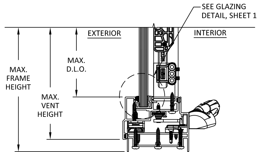
B 3 VERTICAL SECTION SILL DETAIL
