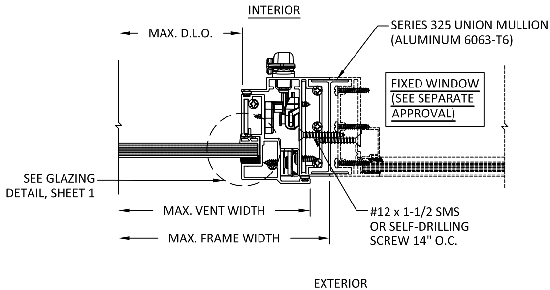
C 4 HORIZONTAL SECTION PROJECT OUT TO FIXED
