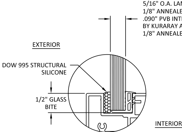
GLAZING DETAIL 1
