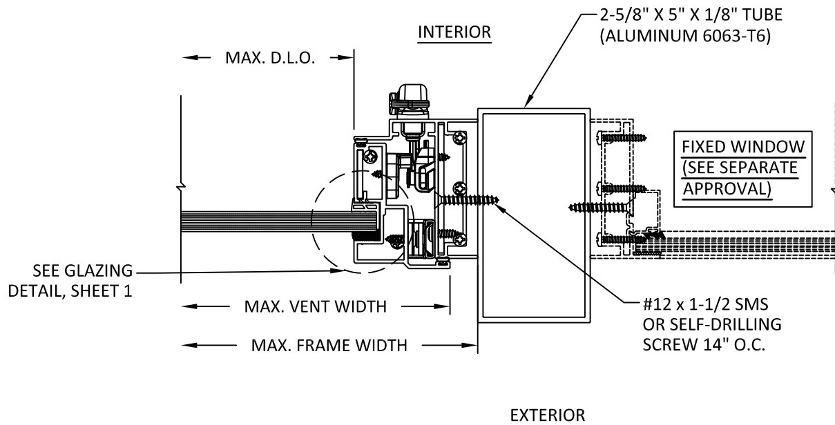
D 4 HORIZONTAL SECTION PROJECT OUT TO FIXED
