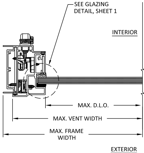
A 4 HORIZONTAL SECTION LEFT JAMB DETAIL
