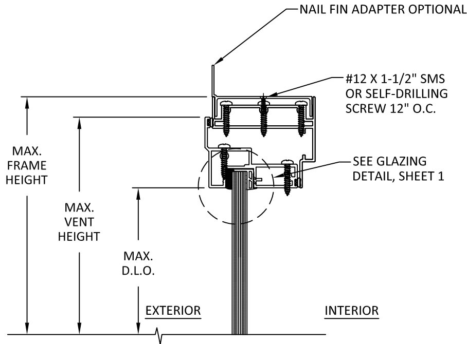
A 3 VERTICAL SECTION HEAD DETAIL NAIL FIN ADAPTER SHOWN
